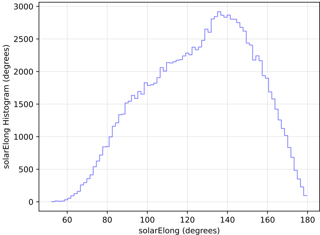
extra_ss_neo7_v3.4_10yrs WFD u band: solarElong Histogram
