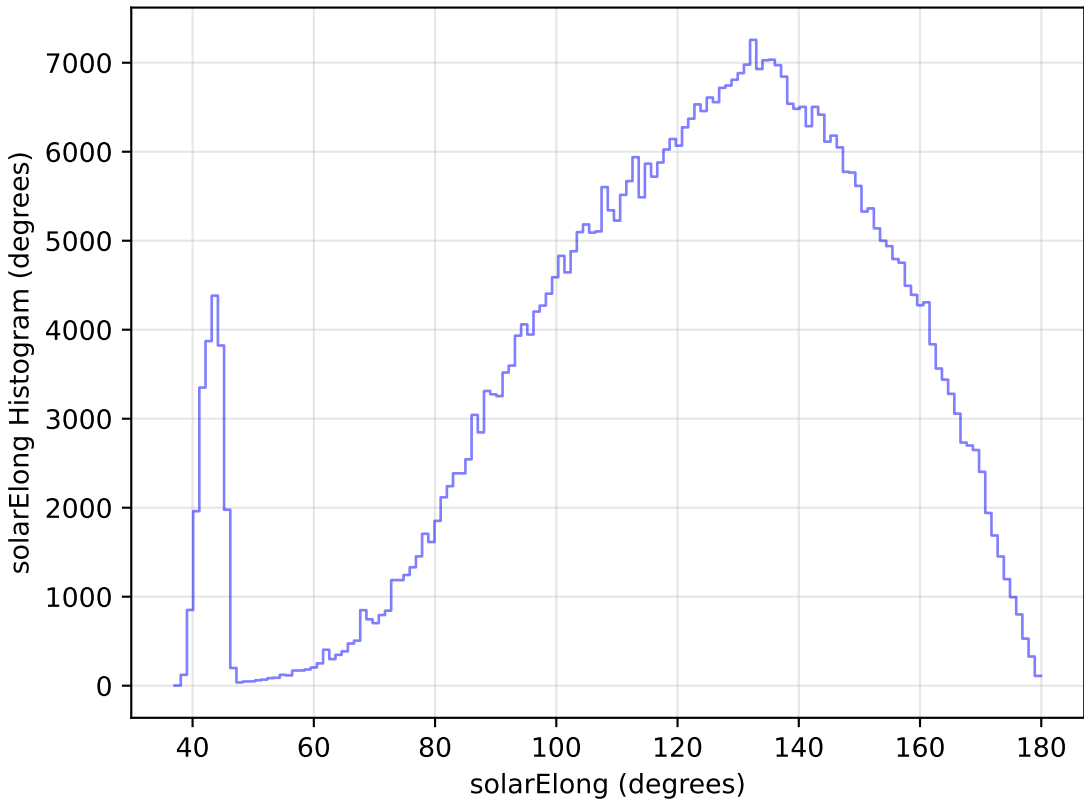
extra_ss_neo7_v3.4_10yrs WFD r band: solarElong Histogram
