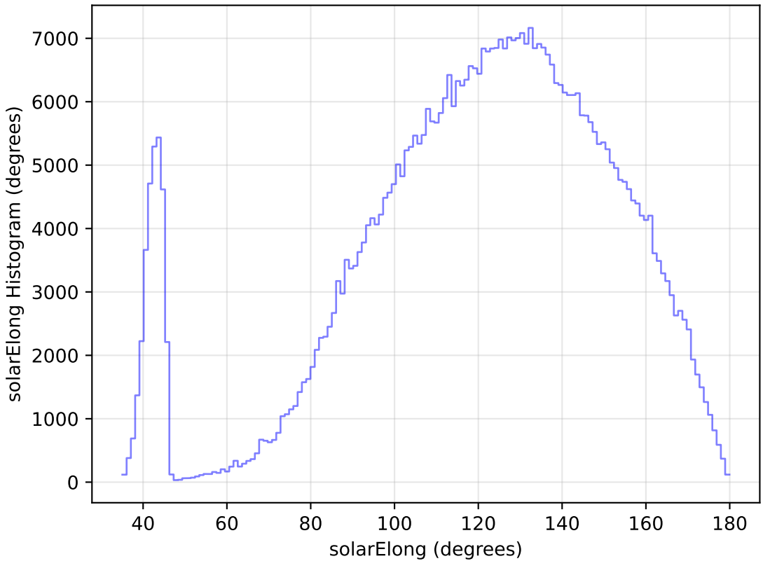
extra_ss_neo7_v3.4_10yrs WFD i band: solarElong Histogram
