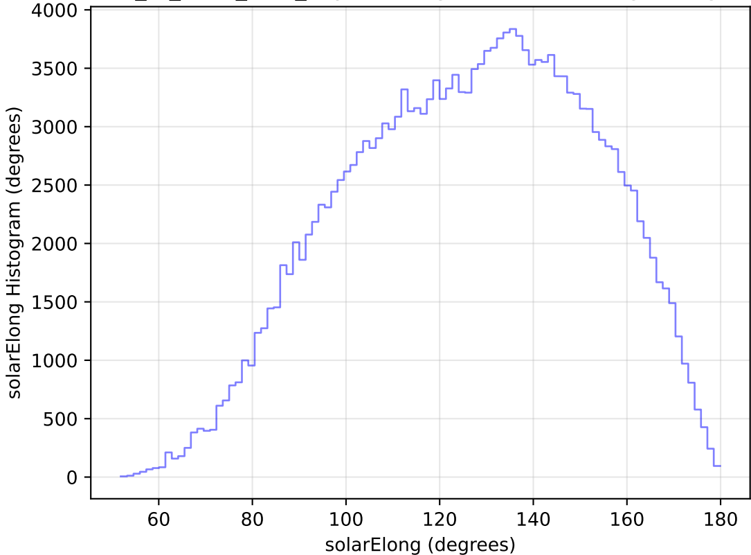
extra_ss_neo7_v3.4_10yrs WFD g band: solarElong Histogram
