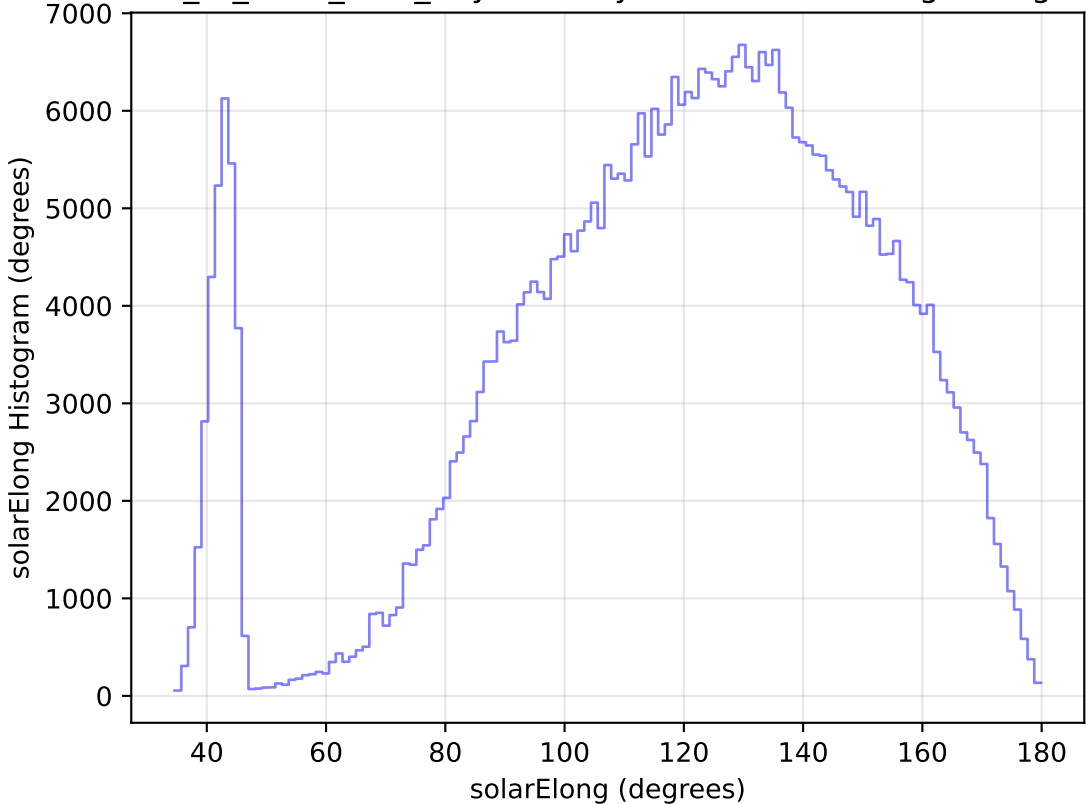
extra_ss_neo7_v3.4_10yrs All sky z band: solarElong Histogram
