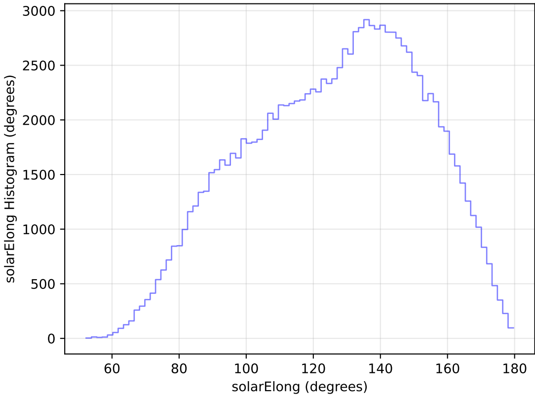
extra_ss_neo7_v3.4_10yrs All sky u band: solarElong Histogram
