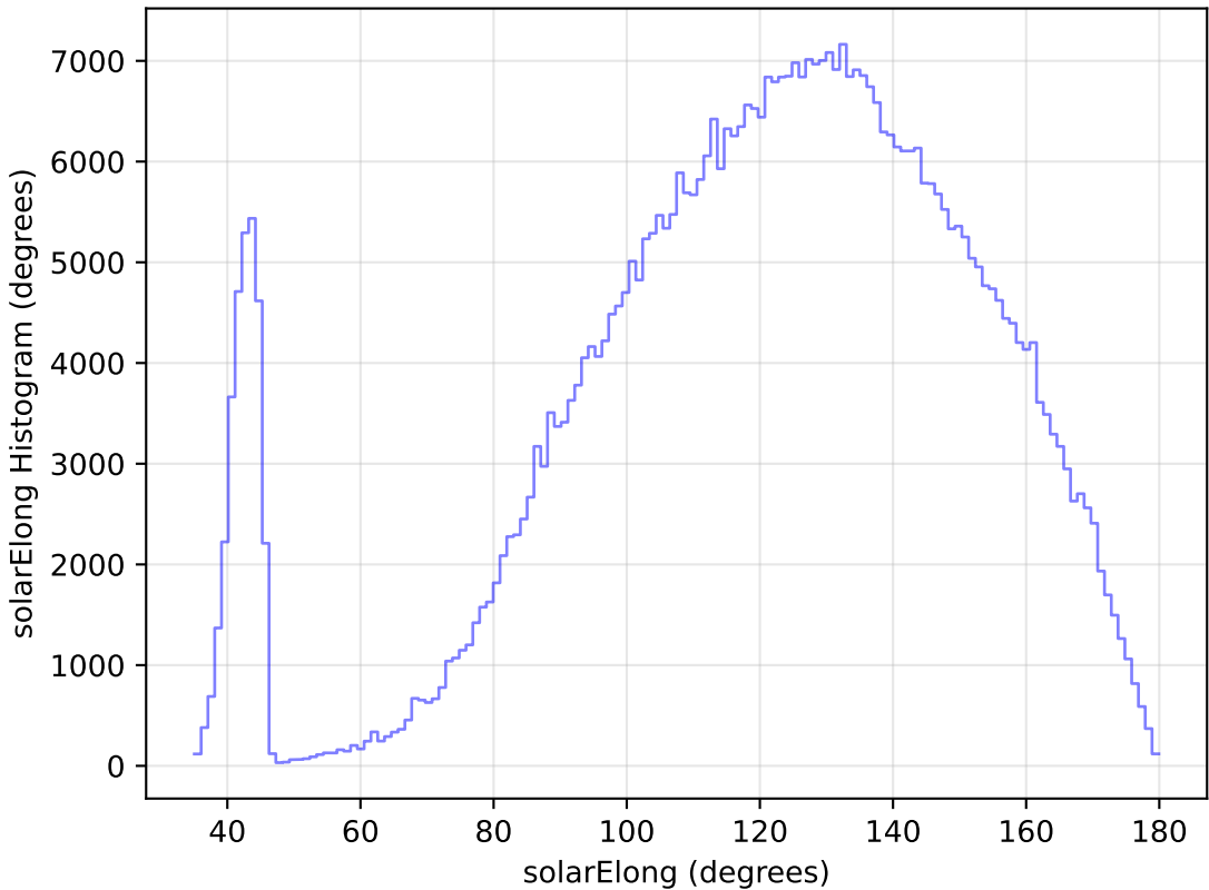
extra_ss_neo7_v3.4_10yrs All sky i band: solarElong Histogram
