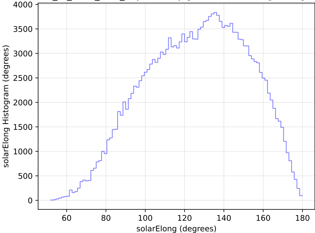
extra_ss_neo7_v3.4_10yrs All sky g band: solarElong Histogram
