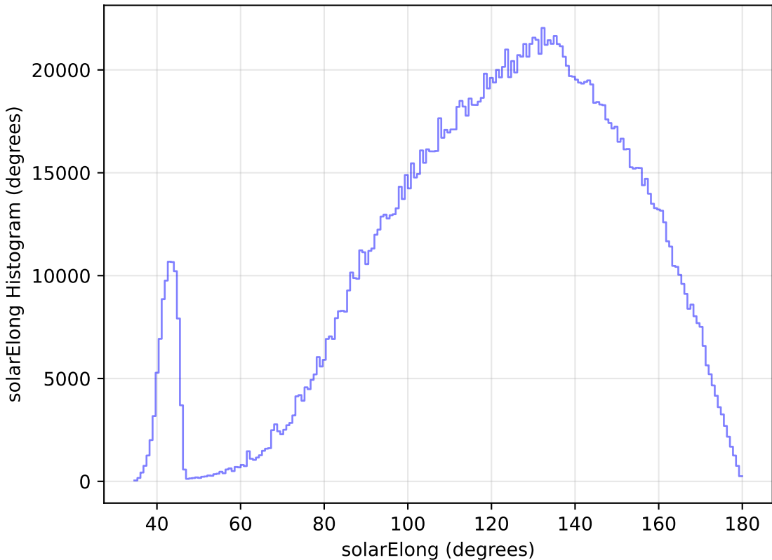
extra_ss_neo7_v3.4_10yrs All sky all bands: solarElong Histogram
