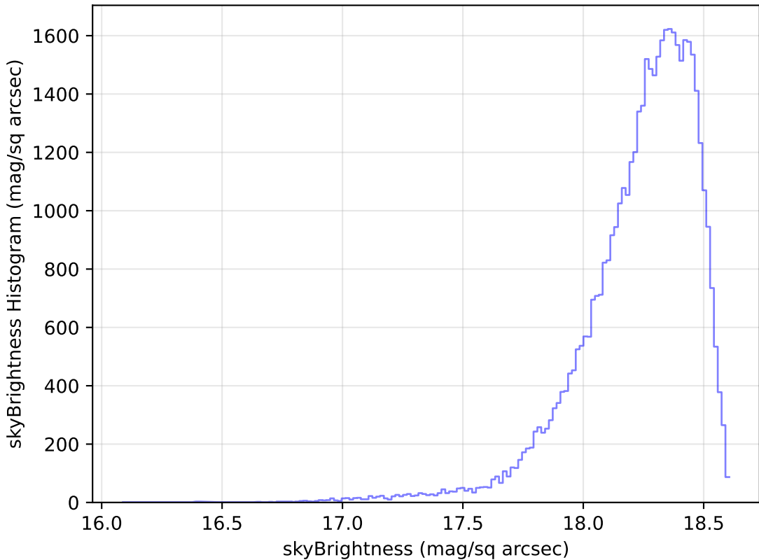
extra_ss_neo7_v3.4_10yrs Yr 1 y band: skyBrightness Histogram
