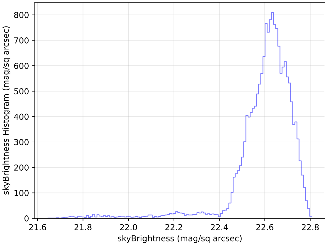
extra_ss_neo7_v3.4_10yrs Yr 1 u band: skyBrightness Histogram
