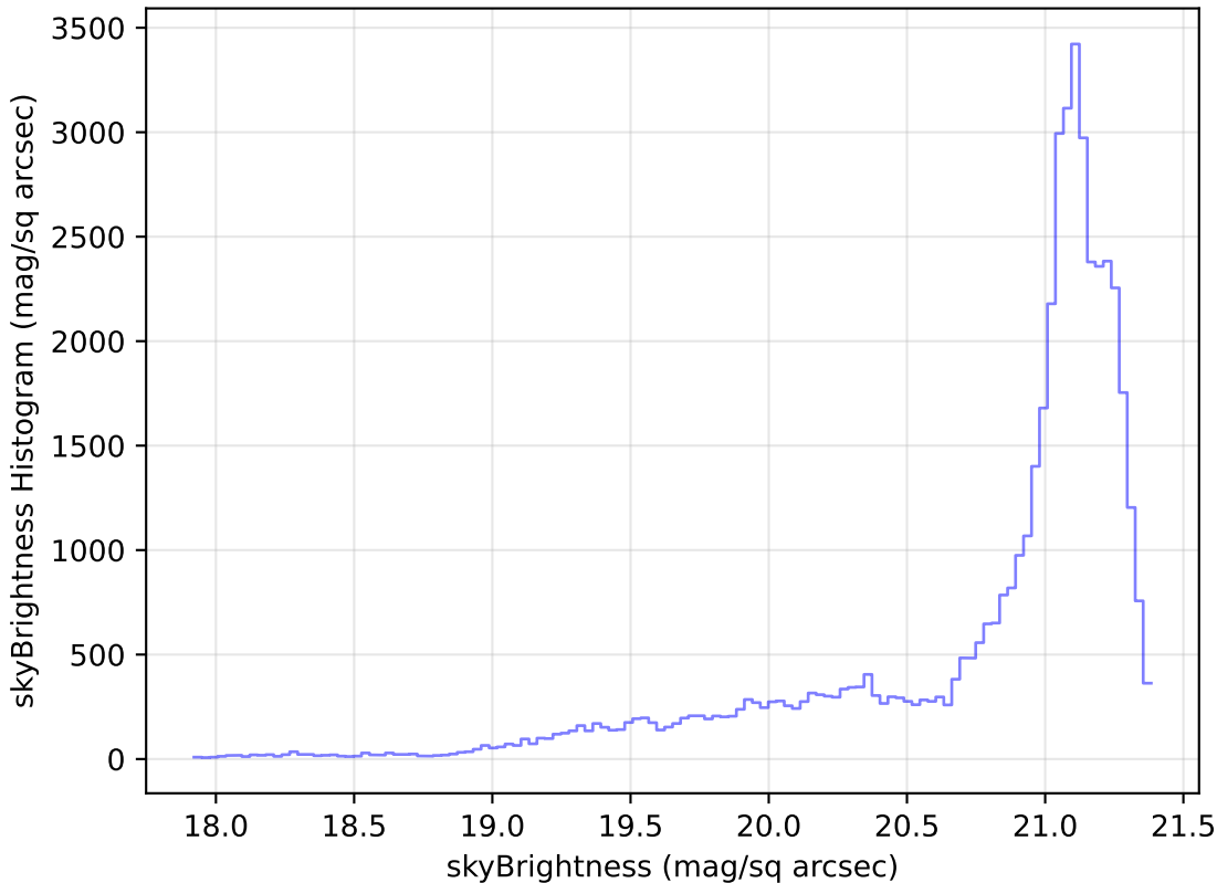
extra_ss_neo7_v3.4_10yrs Yr 1 r band: skyBrightness Histogram
