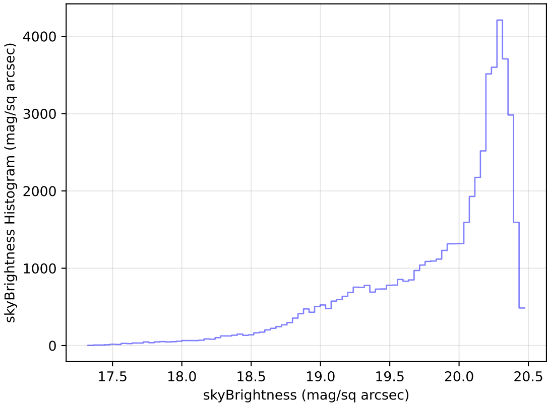
extra_ss_neo7_v3.4_10yrs Yr 1 i band: skyBrightness Histogram
