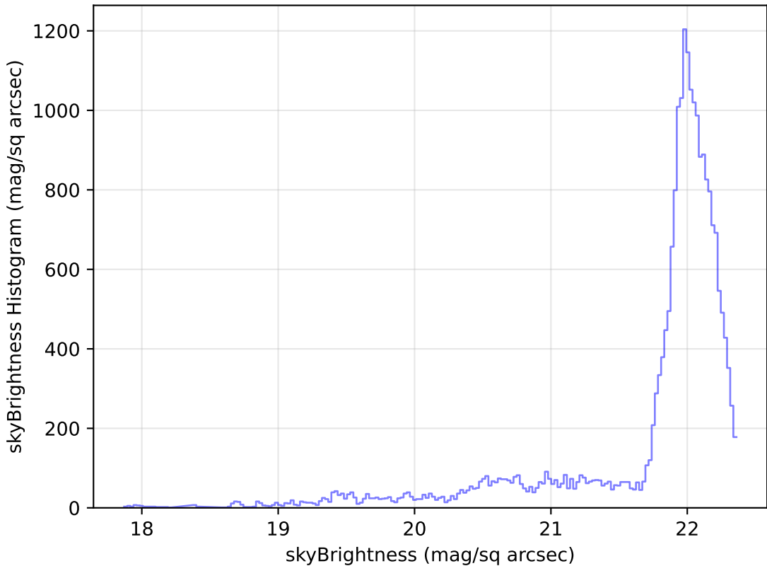
extra_ss_neo7_v3.4_10yrs Yr 1 g band: skyBrightness Histogram
