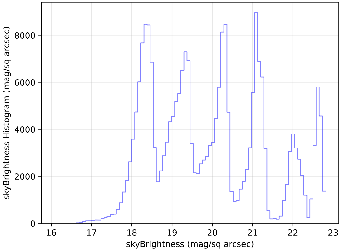
extra_ss_neo7_v3.4_10yrs Yr 1 all bands: skyBrightness Histogram
