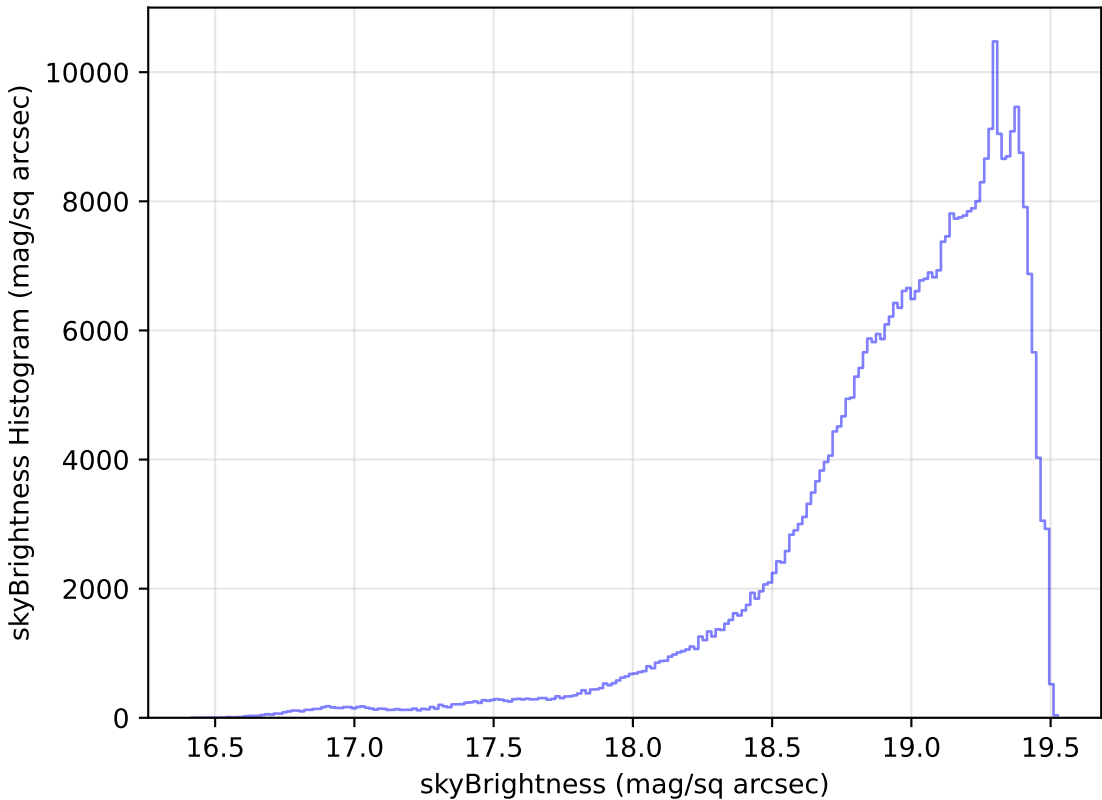
extra_ss_neo7_v3.4_10yrs WFD z band: skyBrightness Histogram
