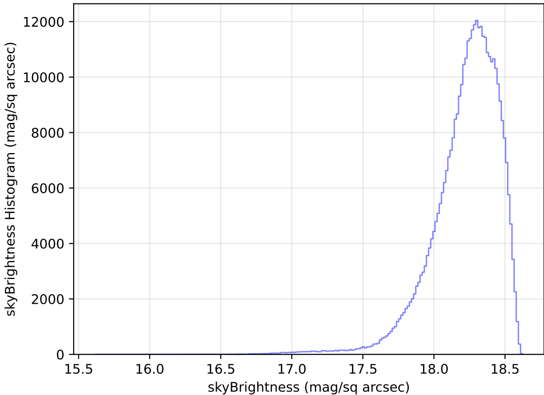
extra_ss_neo7_v3.4_10yrs WFD y band: skyBrightness Histogram
