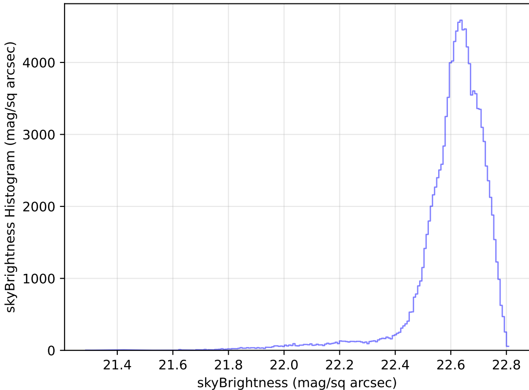
extra_ss_neo7_v3.4_10yrs WFD u band: skyBrightness Histogram
