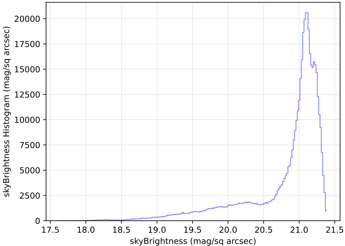
extra_ss_neo7_v3.4_10yrs WFD r band: skyBrightness Histogram
