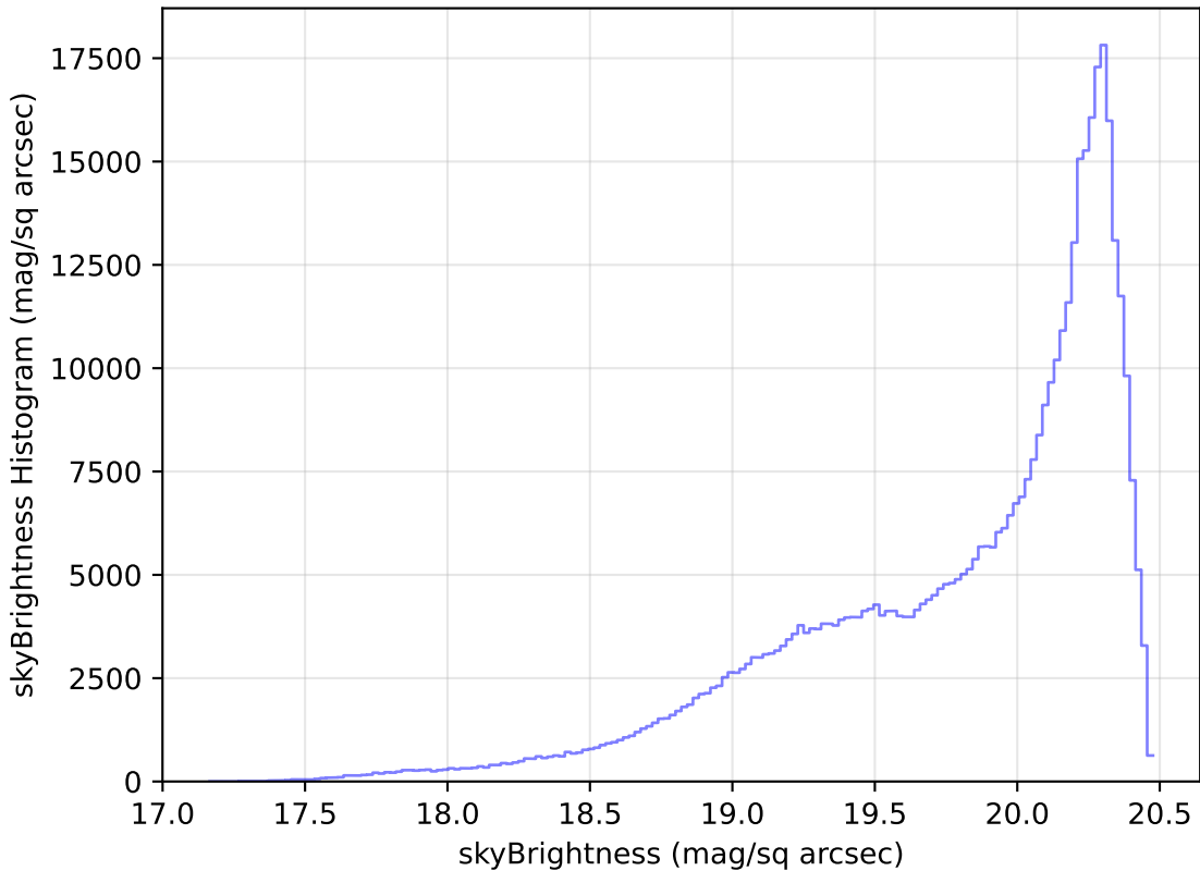
extra_ss_neo7_v3.4_10yrs WFD i band: skyBrightness Histogram
