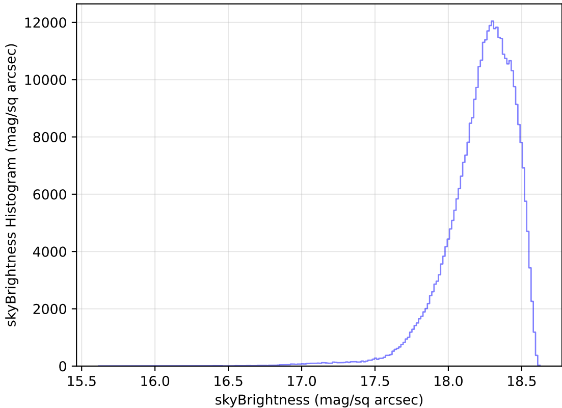
extra_ss_neo7_v3.4_10yrs All sky y band: skyBrightness Histogram
