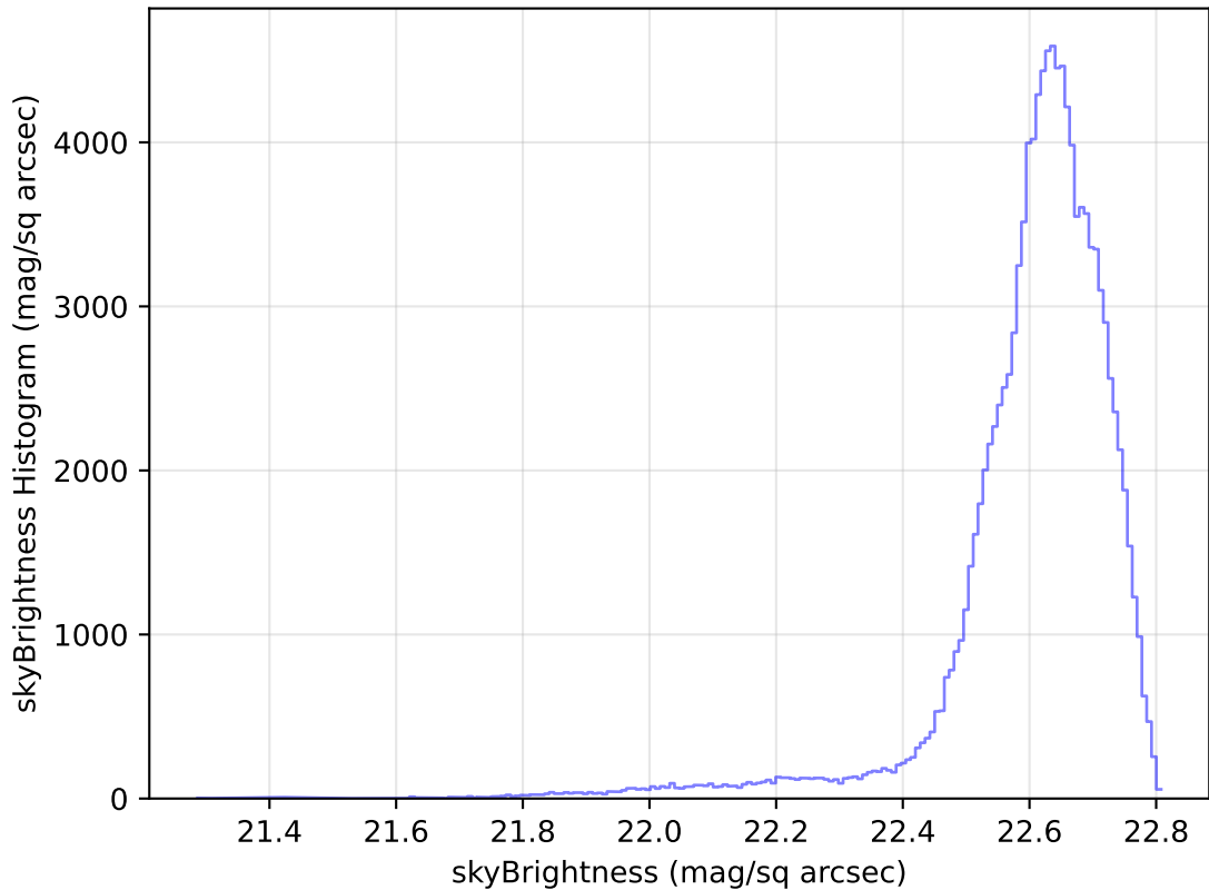
extra_ss_neo7_v3.4_10yrs All sky u band: skyBrightness Histogram
