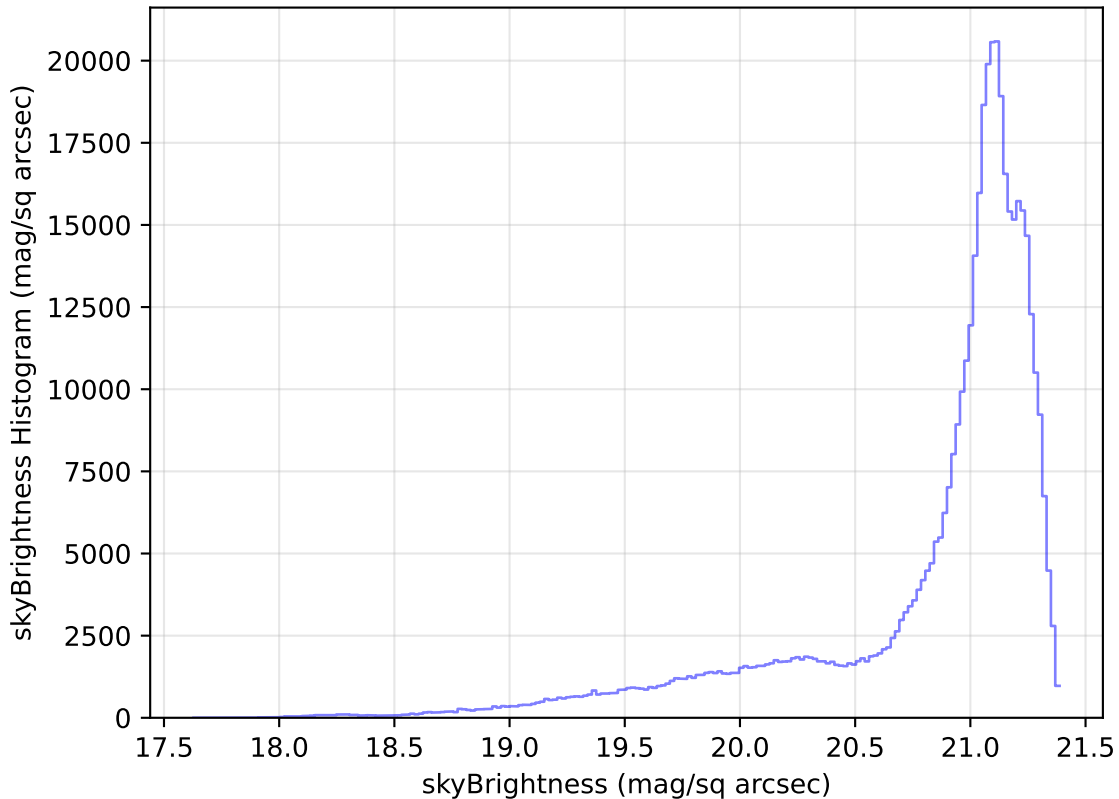
extra_ss_neo7_v3.4_10yrs All sky r band: skyBrightness Histogram
