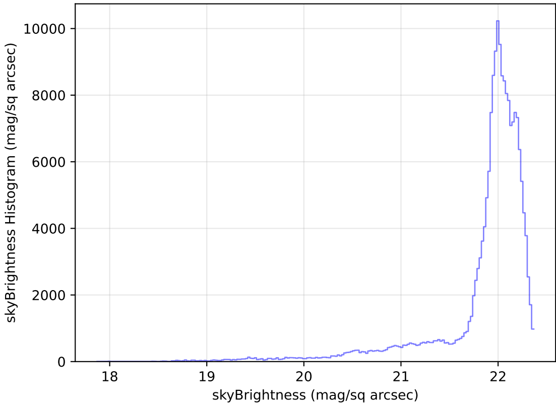
extra_ss_neo7_v3.4_10yrs All sky g band: skyBrightness Histogram
