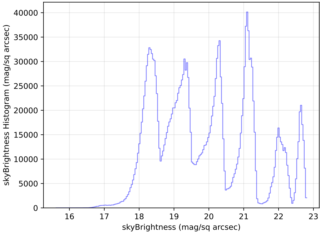
extra_ss_neo7_v3.4_10yrs All sky all bands: skyBrightness Histogram
