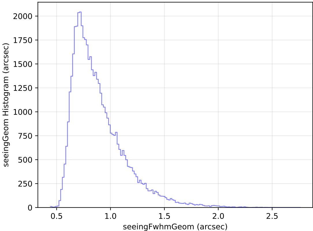
extra_ss_neo7_v3.4_10yrs Yr 1 r band: seeingGeom Histogram
