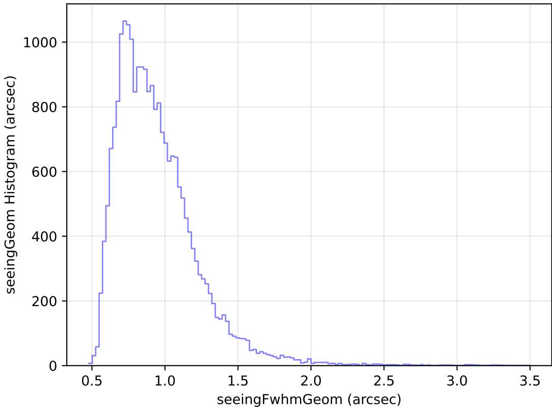
extra_ss_neo7_v3.4_10yrs Yr 1 g band: seeingGeom Histogram
