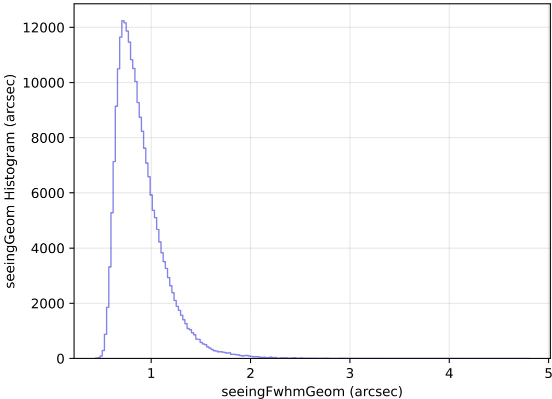
extra_ss_neo7_v3.4_10yrs Yr 1 all bands: seeingGeom Histogram
