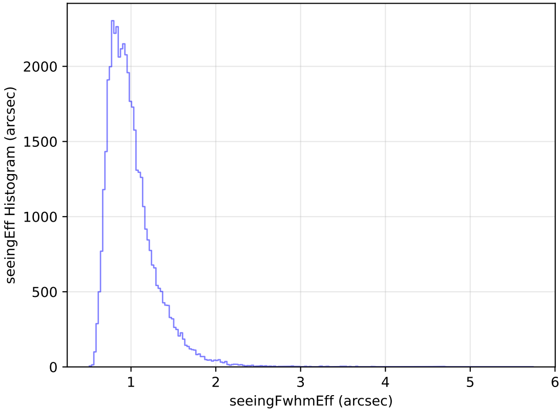
extra_ss_neo7_v3.4_10yrs Yr 1 z band: seeingEff Histogram
