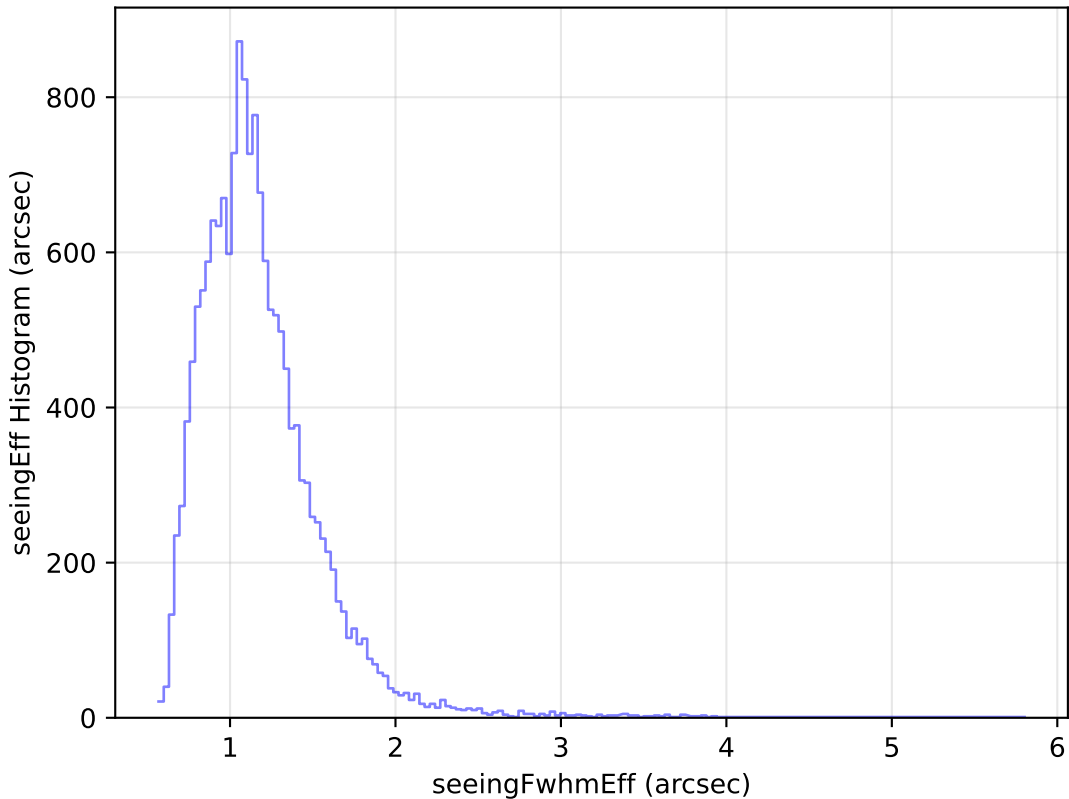
extra_ss_neo7_v3.4_10yrs Yr 1 u band: seeingEff Histogram
