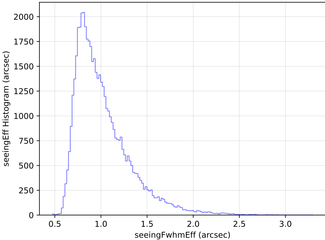
extra_ss_neo7_v3.4_10yrs Yr 1 r band: seeingEff Histogram
