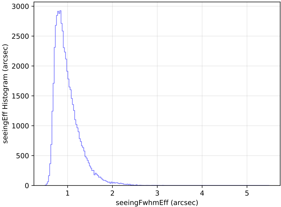
extra_ss_neo7_v3.4_10yrs Yr 1 i band: seeingEff Histogram
