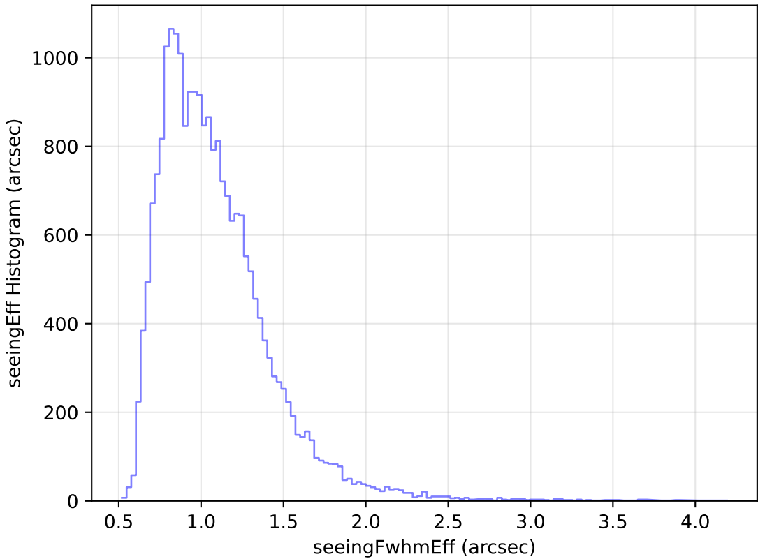
extra_ss_neo7_v3.4_10yrs Yr 1 g band: seeingEff Histogram
