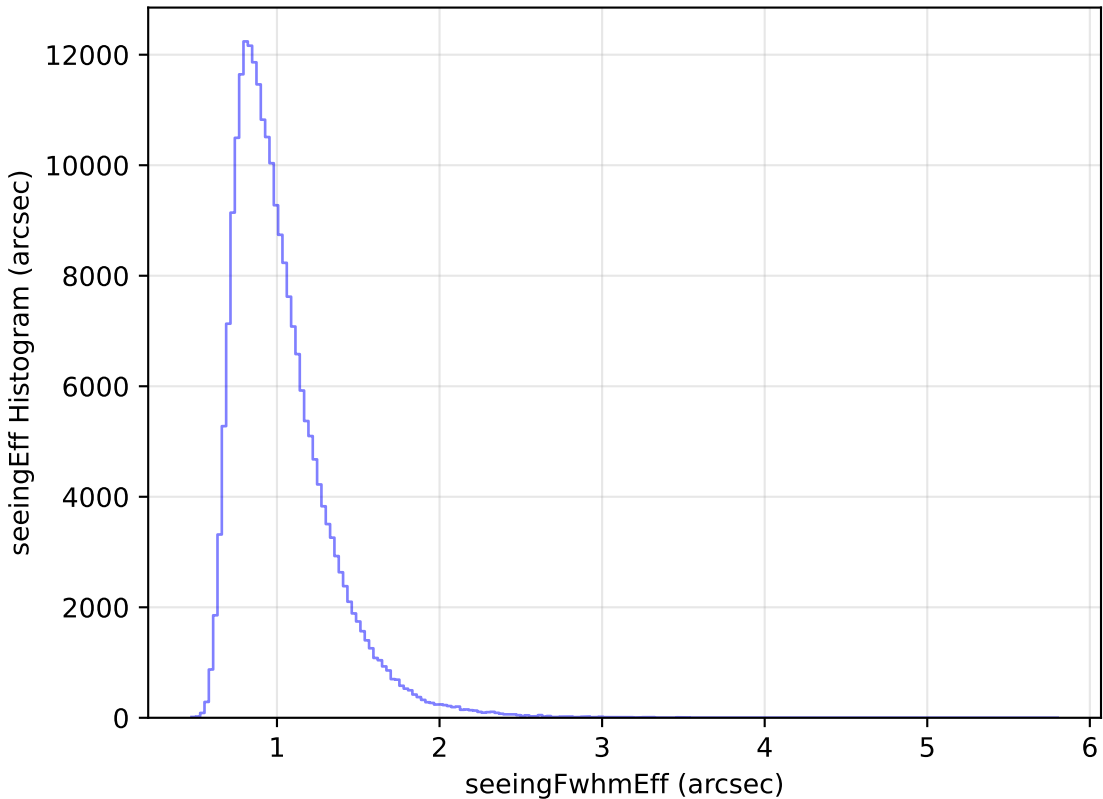
extra_ss_neo7_v3.4_10yrs Yr 1 all bands: seeingEff Histogram
