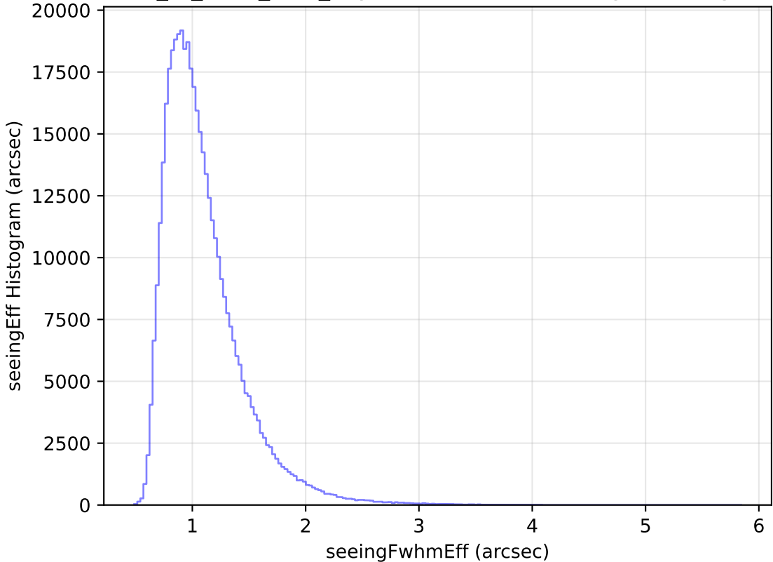
extra_ss_neo7_v3.4_10yrs WFD z band: seeingEff Histogram
