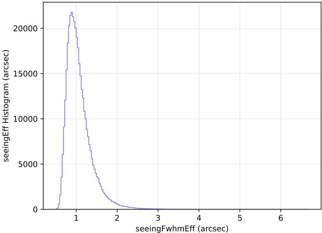
extra_ss_neo7_v3.4_10yrs WFD y band: seeingEff Histogram
