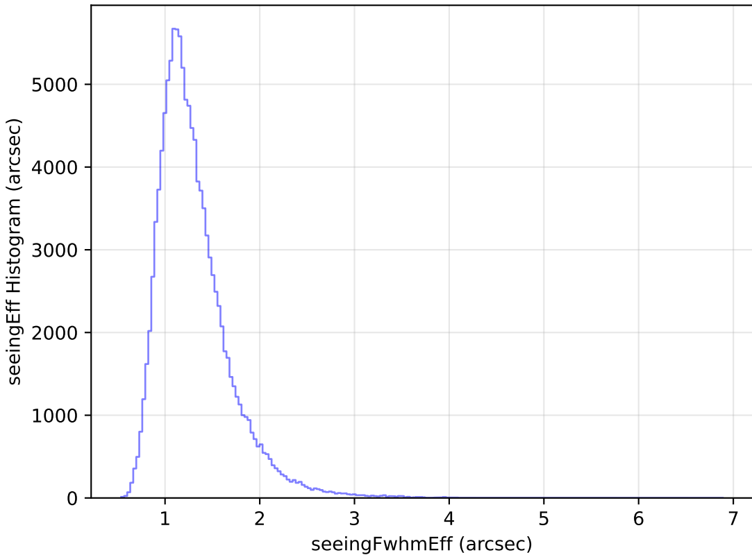
extra_ss_neo7_v3.4_10yrs WFD u band: seeingEff Histogram
