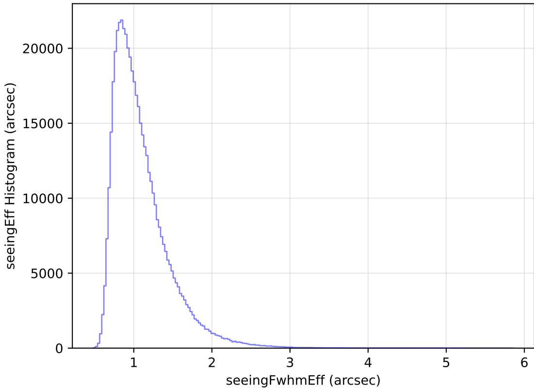
extra_ss_neo7_v3.4_10yrs WFD i band: seeingEff Histogram
