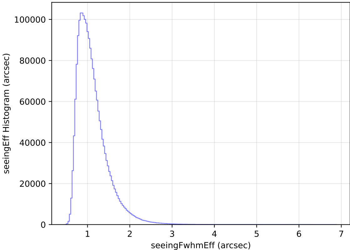
extra_ss_neo7_v3.4_10yrs WFD all bands: seeingEff Histogram
