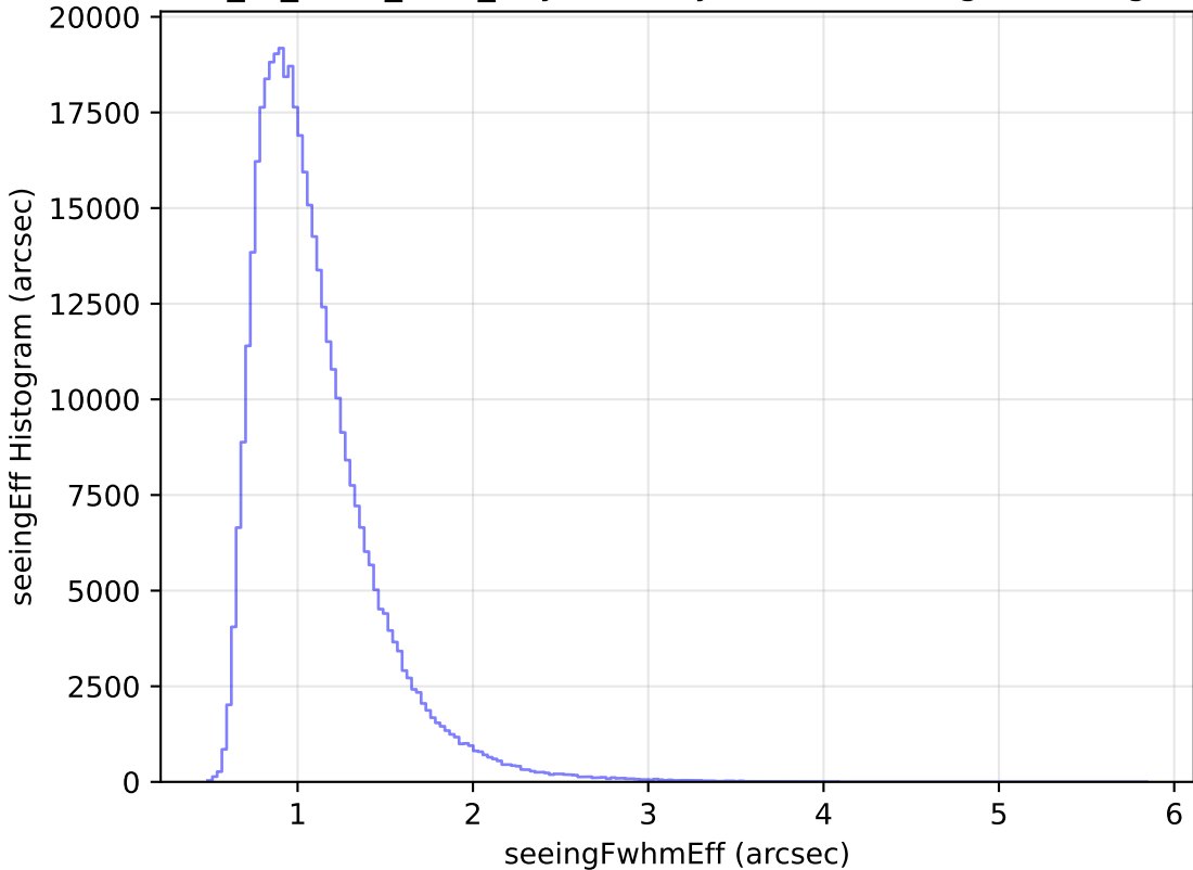
extra_ss_neo7_v3.4_10yrs All sky z band: seeingEff Histogram
