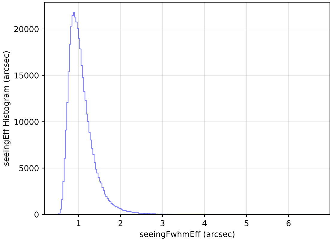
extra_ss_neo7_v3.4_10yrs All sky y band: seeingEff Histogram
