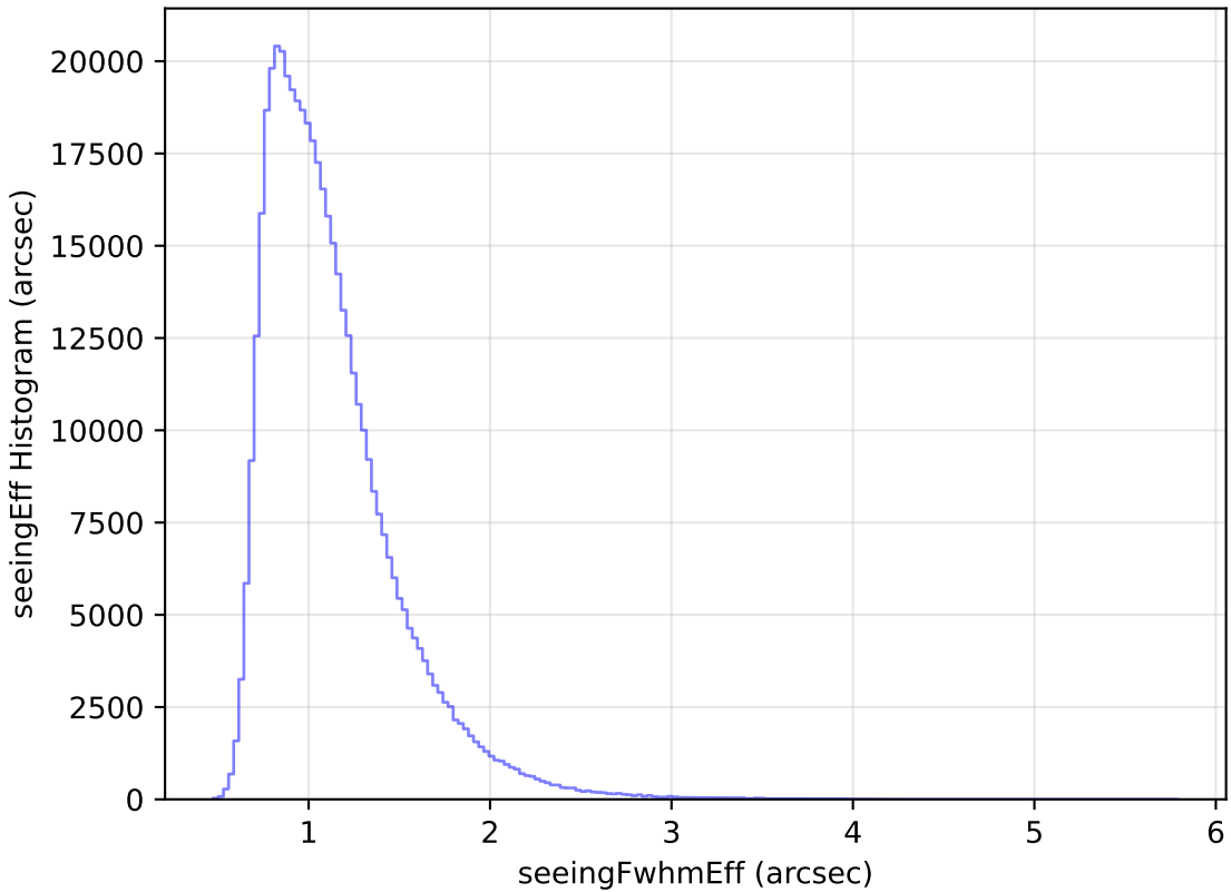
extra_ss_neo7_v3.4_10yrs All sky r band: seeingEff Histogram
