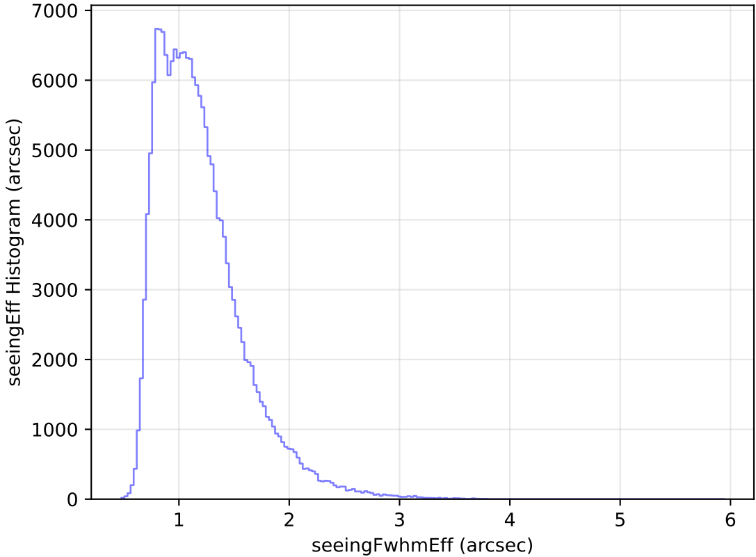
extra_ss_neo7_v3.4_10yrs All sky g band: seeingEff Histogram
