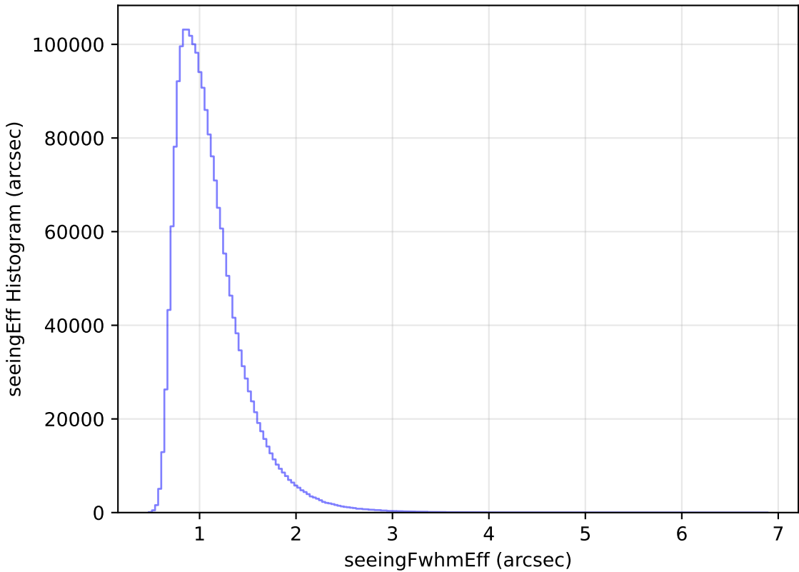
extra_ss_neo7_v3.4_10yrs All sky all bands: seeingEff Histogram
