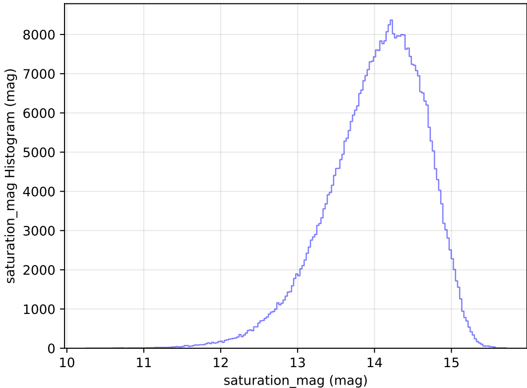
extra_ss_neo7_v3.4_10yrs WFD z band: saturation_mag Histogram
