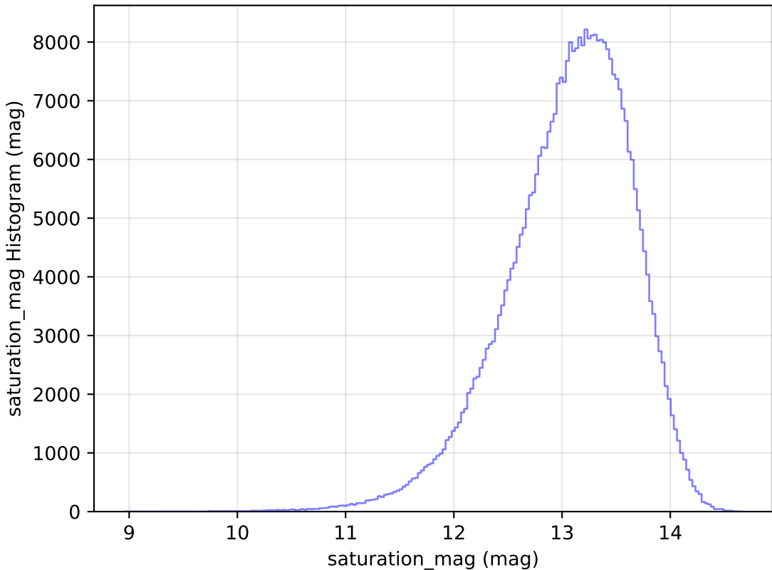
extra_ss_neo7_v3.4_10yrs WFD y band: saturation_mag Histogram
