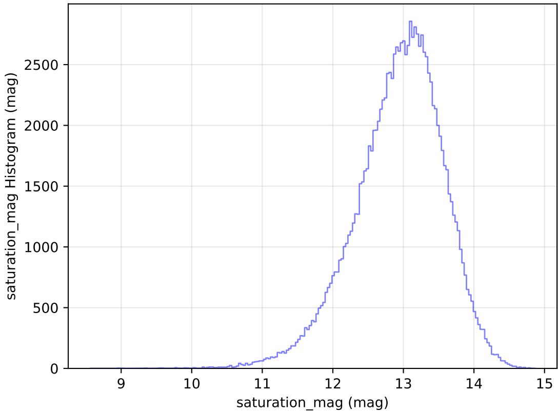
extra_ss_neo7_v3.4_10yrs WFD u band: saturation_mag Histogram
