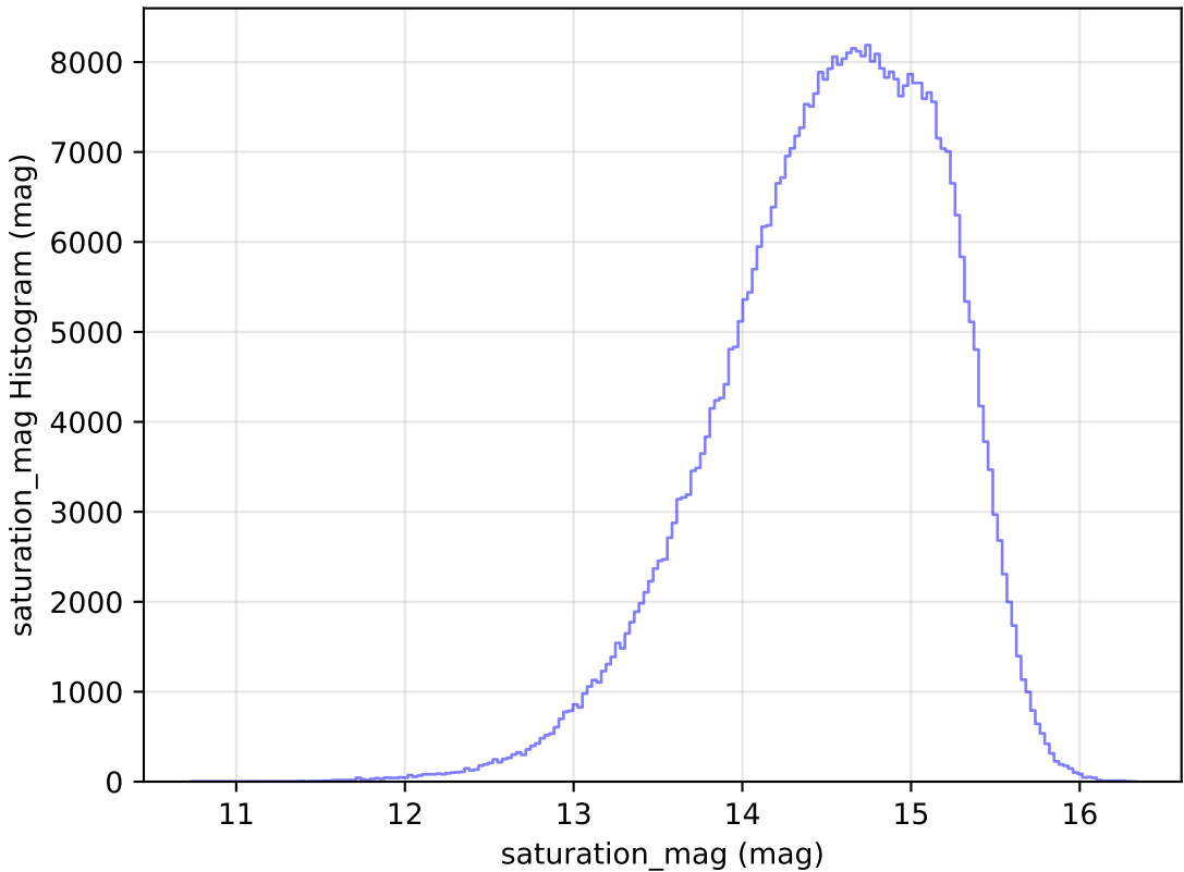
extra_ss_neo7_v3.4_10yrs WFD r band: saturation_mag Histogram
