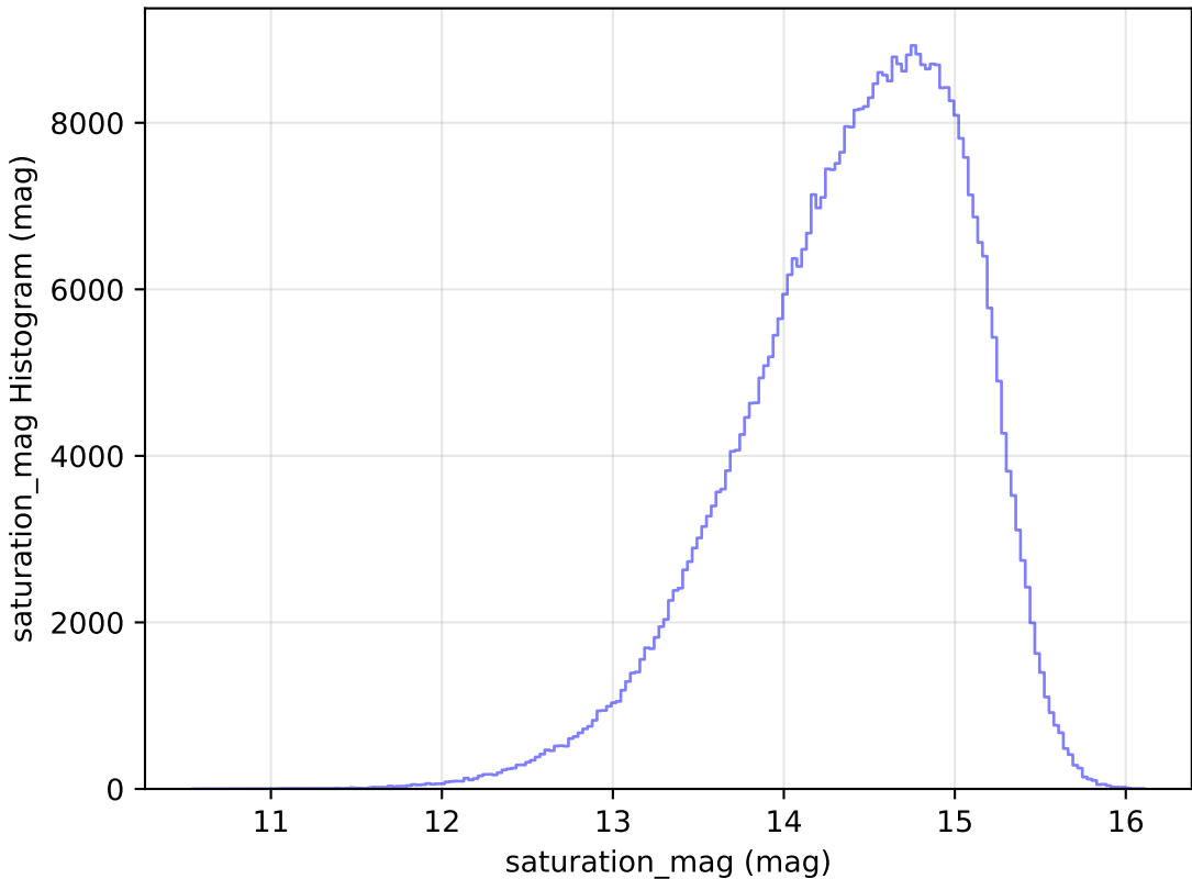
extra_ss_neo7_v3.4_10yrs WFD i band: saturation_mag Histogram
