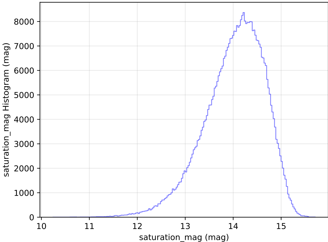
extra_ss_neo7_v3.4_10yrs All sky z band: saturation_mag Histogram
